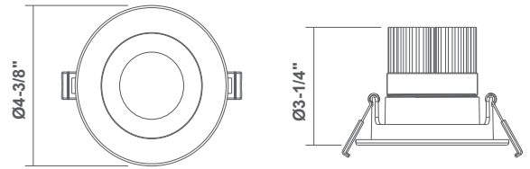
3.5" LED Regress Gimbal - Round
