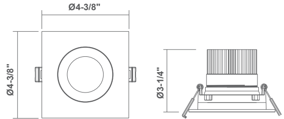
3.5" LED Regress Gimbal - Square
